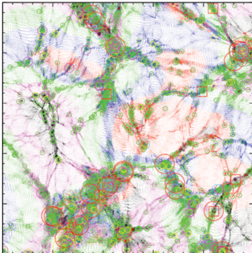
Halo-finding algorithm identifies dense concentrations of particles that are gravitationally bound to one another. Dark-matter halos are the sites where galaxies live; they are called halos because they extend beyond the perimeter of the galaxy. Since the Bolshoi simulation includes only dark matter, the galaxies themselves are not explicitly present. In this thin slice through the final state of the Bolshoi simulation, halos with various properties are marked by circles and polygons. Just as individual particles fall together to form halos, the halos also tend to merge, forming a nested hierarchy. The image was created by Stefan Gottlöber.
