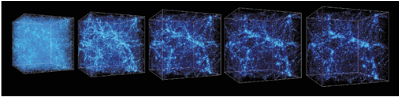
Snapshots from the evolution of a simulated universe show the gradual emergence of large-scale structures as particles come together under their mutual gravitational attraction. In the leftmost panel the initial state of the system, representing a moment roughly 100 million years after the Big Bang, has particles distributed almost uniformly, with only slight fluctuations in density. Over the subsequent 13 billion years the particle population condenses in filaments, some of which extend across the entire volume. The rightmost panel shows the final configuration. The illustration is not from the Bolshoi project but from an earlier simulation carried out at the National Center for Supercomputer Applications by Andrey V. Kravtsov of the University of Chicago and Anatoly Klypin of New Mexico State University. The visualization was created by Kravtsov.
